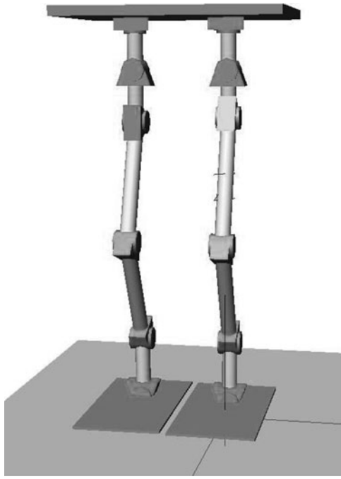
Fig. 2. Biped model of MANUS-I in visualNastran 4D environment.
