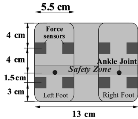
Fig. 6. Positions of the foot sensors at the bottom of the feet.
