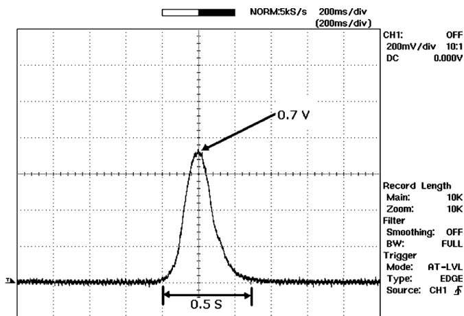
Fig. 14. Oscilloscope display of the applied force.
