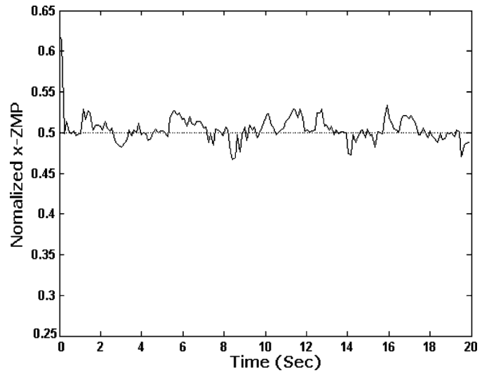
Fig. 11. Normalized x-ZMP Position of Compensated Walking Gait.
