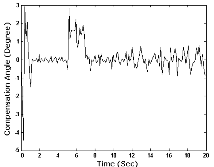
Fig. 16. Compensation at the ankle-joint of MANUS-I to compensate a sudden push of intensity around 3 N from behind.
