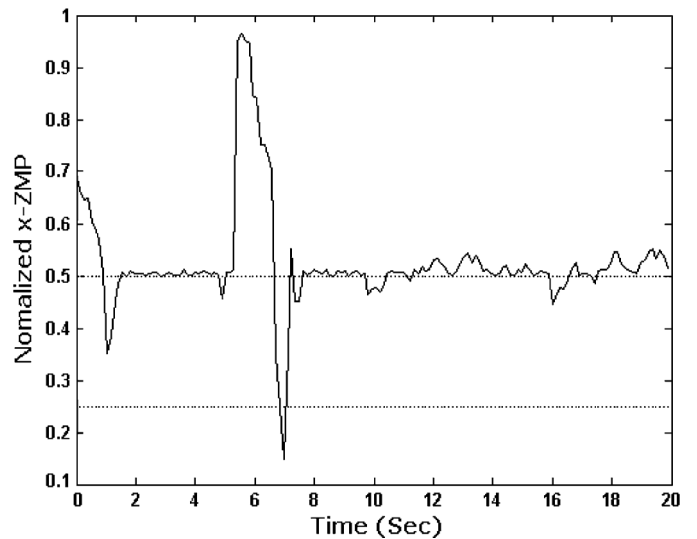
Fig. 15. Normalized x-ZMP Position of MANUS-I when it experience a sudden push of intensity around 3 N from behind.
