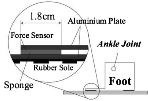
Fig. 4. Mechanical installation of force sensors.
