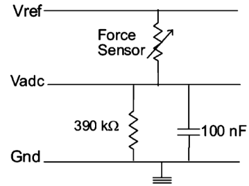
Fig. 5. Force-to-Voltage converter circuit.
